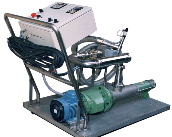
Dosage equipment with progressive cavity pump, turbine flow meter and programmer
