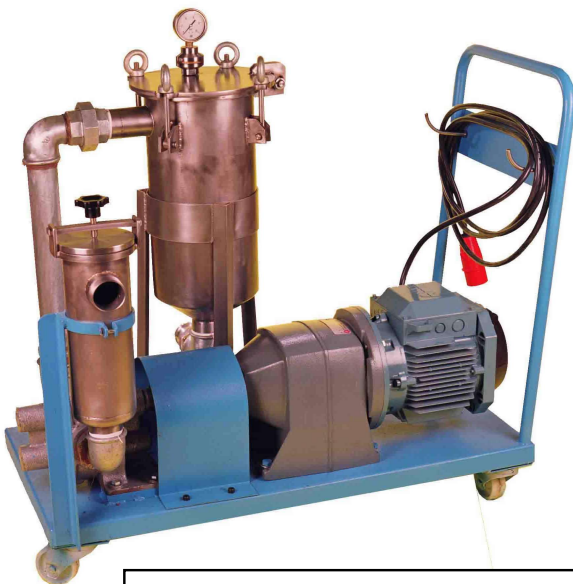
Gear pump with 2" pre-filter and 2" bag filter
