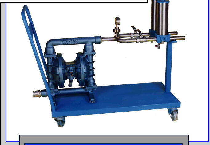
Circulation equipment with membrane pump made of 1 1/2" aluminium-Teflon and two short cuno filters (10")
