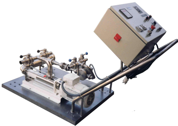
Dosage equipment with progressive cavity pump, oval gear flow meter and programmer
