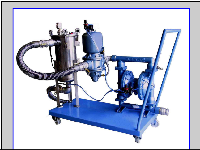
Circulation equipment with membrane pump, anti-pulse device and bag filter
